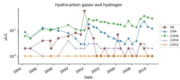
Figure 5: Chart of hydrogen and hydrocarbon gases.
