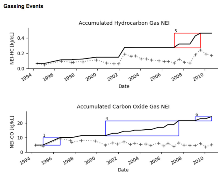
Figure 6: Fault energy index charts with gassing events indicated by colored boxes.
