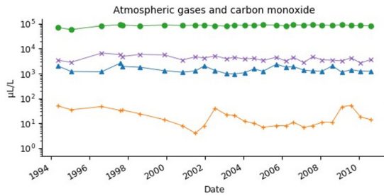
Figure 4: Chart of atmospheric and carbon oxide gases.
